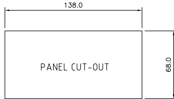
CUT-OUT DETAILS FOR PANEL MOUNTING
